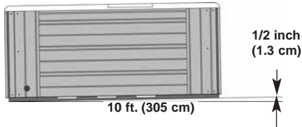
Slope 1/2 inch per 10 ft. for proper drainage.
