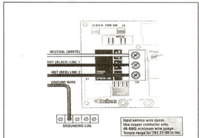
Printed Circuit Board Layout
